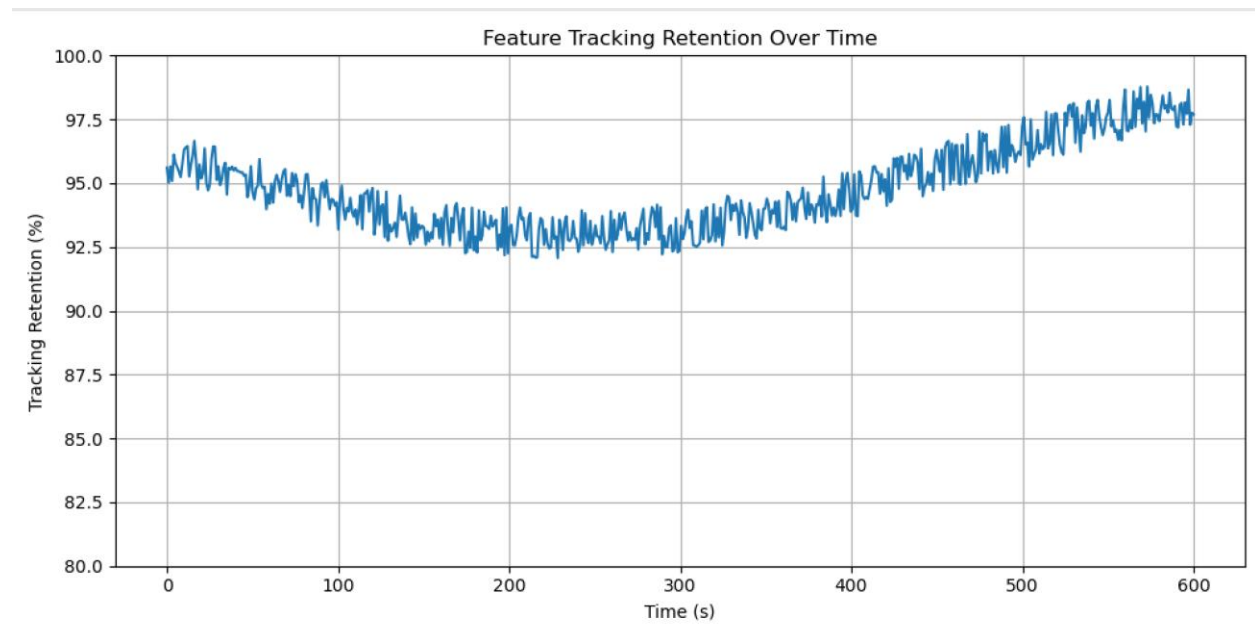
Fig. 9. Feature tracking retention over time. Feature-tracking retention curves across the evaluation sequence. AUROADAS maintains consistently high retention (91–98%) due to transformer-derived global context, which stabilizes feature identity under occlusion and dynamic motion. A brief mid-sequence dip corresponds to increased environmental complexity, followed by rapid recovery enabled by sparse attention, token-reduction focusing, and fused ego-pose stabilization.
